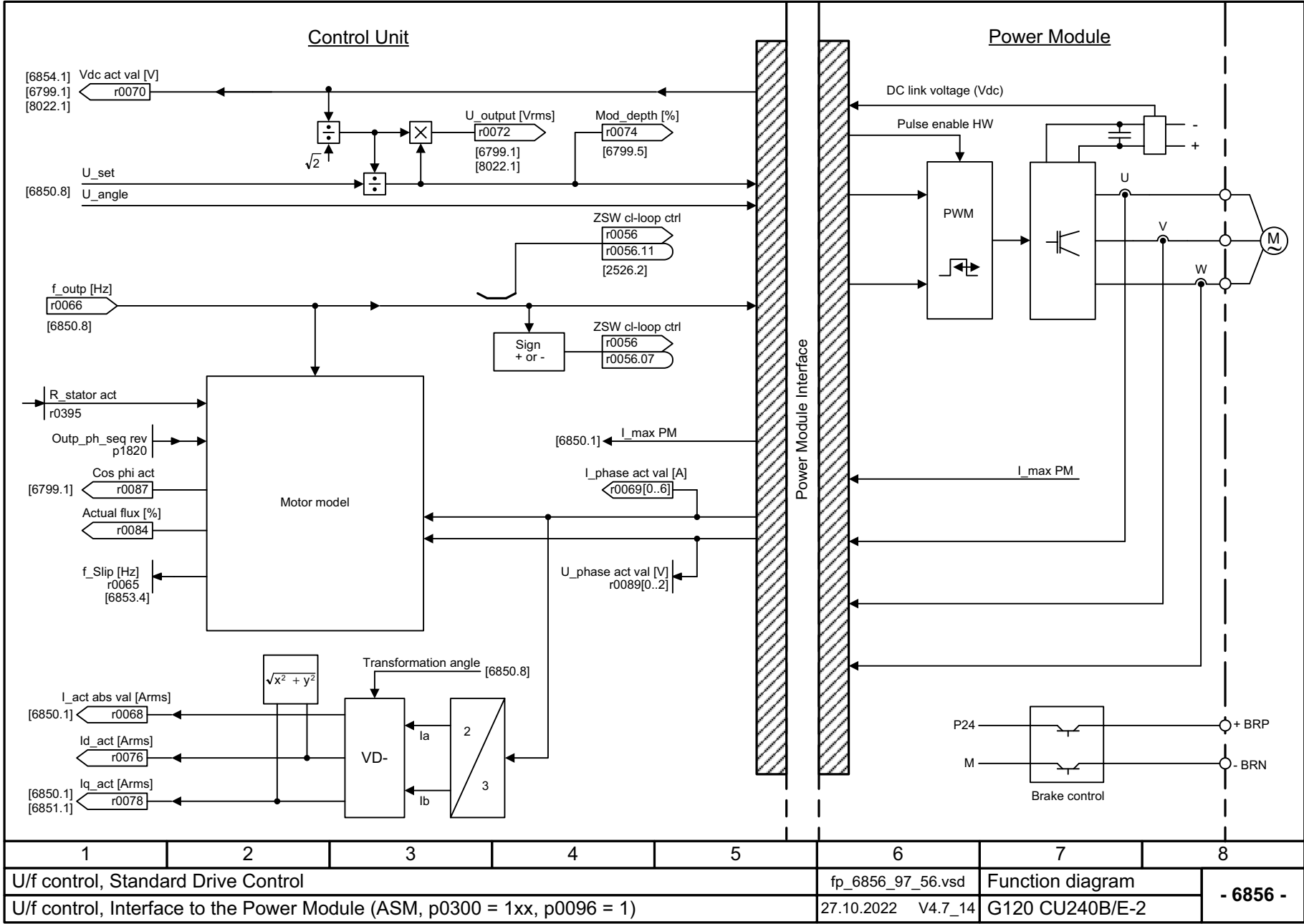
图 3-122 6856 - 和功率模块的接口 (ASM, p0300 = 1, p0096 = 1)
