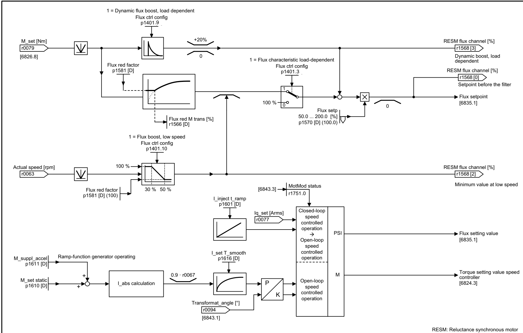
图 3-133 6834 - 磁通设定值 (RESM, p0300 = 6xx, p0096 = 2)
