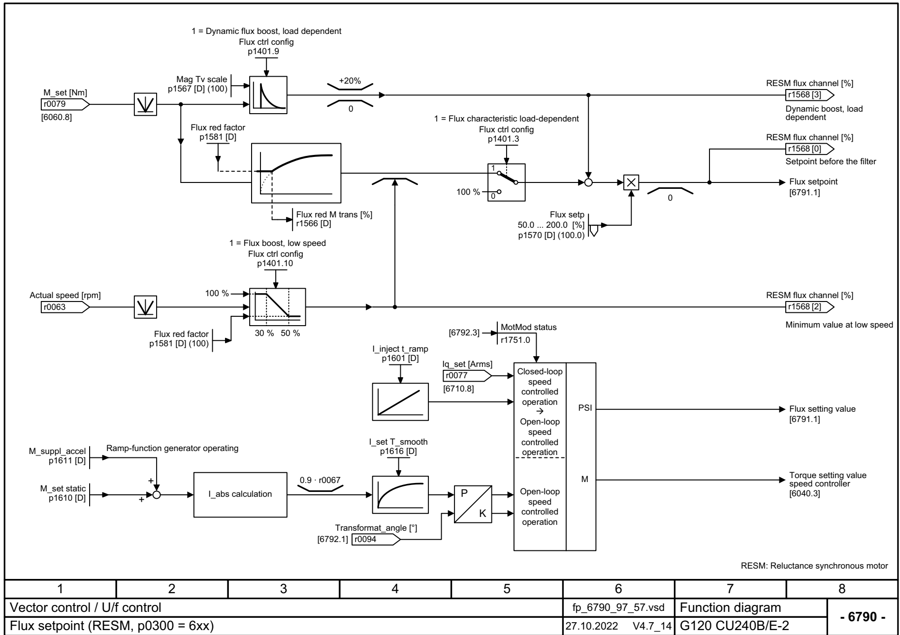
图 3-114 6790 - 磁通设定值 (RESM, p0300 = 6xx)
