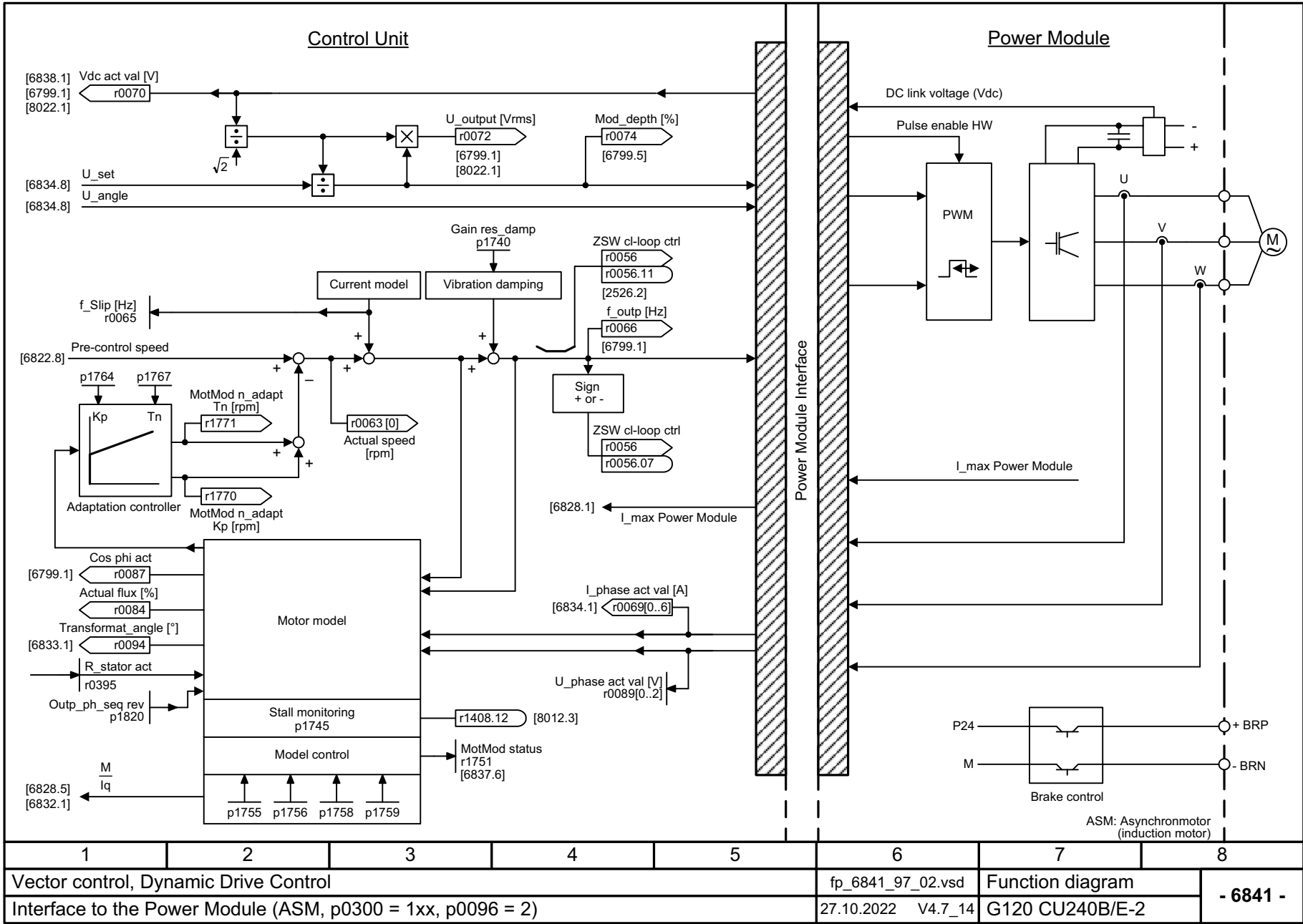
图 3-139 6841 - 到功率模块的接口 (ASM, p0300 = 1, p0096 = 2)
