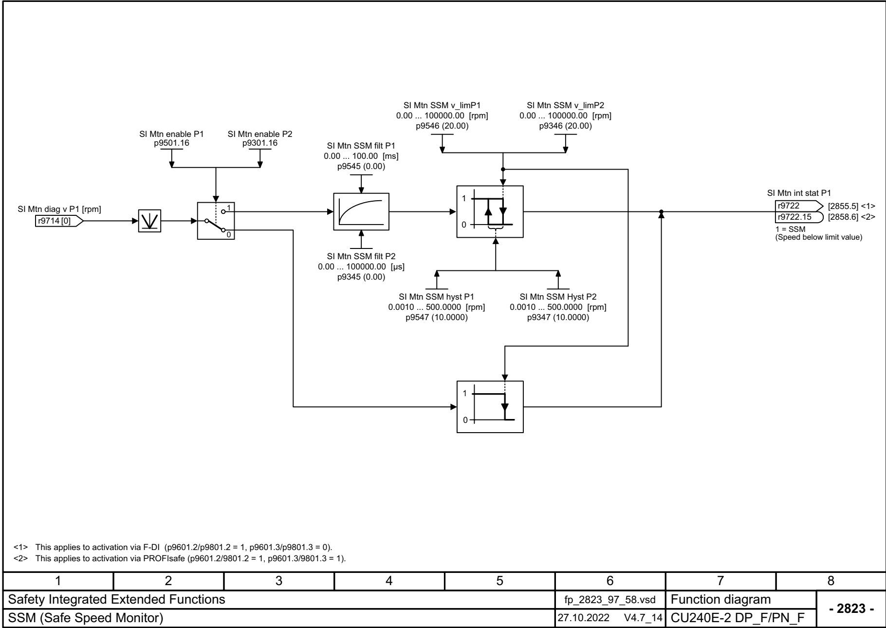
图 3-70 2823 - SSM (Safe Speed Monitor)
